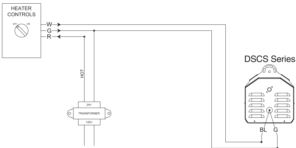
Figure 2 • Single Stage Wiring for Single Heater (TH-DSSS1)
