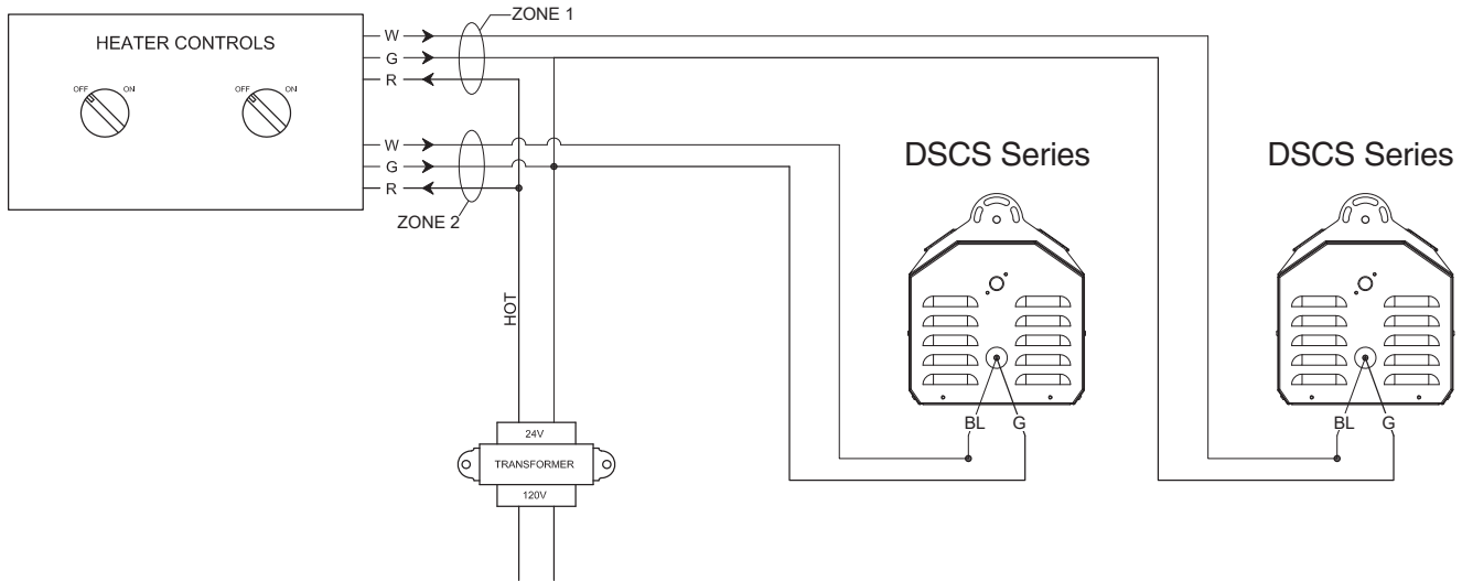
Figure 3 • Single Stage Wiring for Multiple Heaters (TH-DSSS2)
